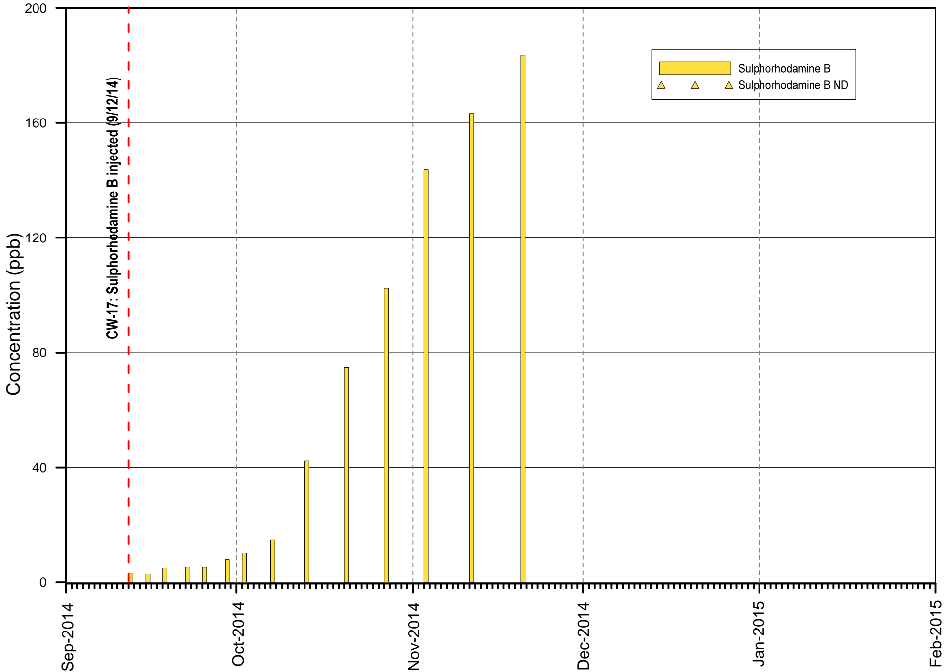
Figure 3.2-7 MW-98S Dye Tracer Analysis Sulphorhodamine B Detections - 2nd Test at CW-17
